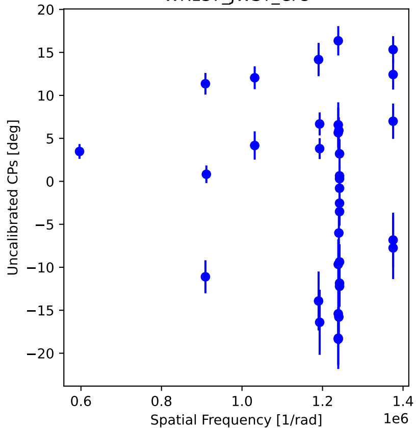
WR137_JWST_CP s
