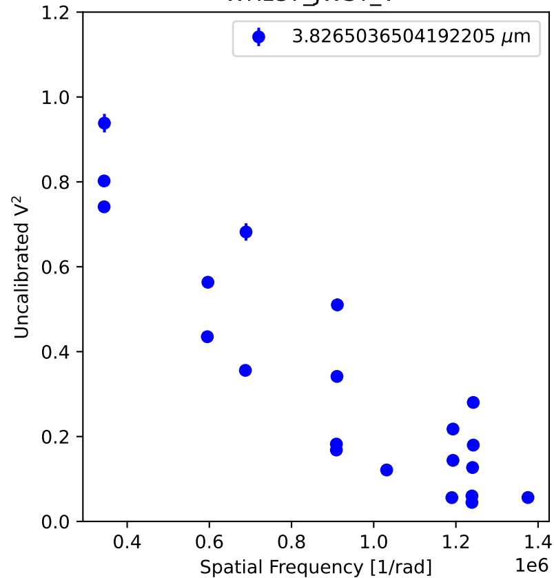
WR137_JWST_V 2
